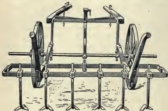
FIG. 3.—Martin's General Purpose Steerage Horse Hoe.
